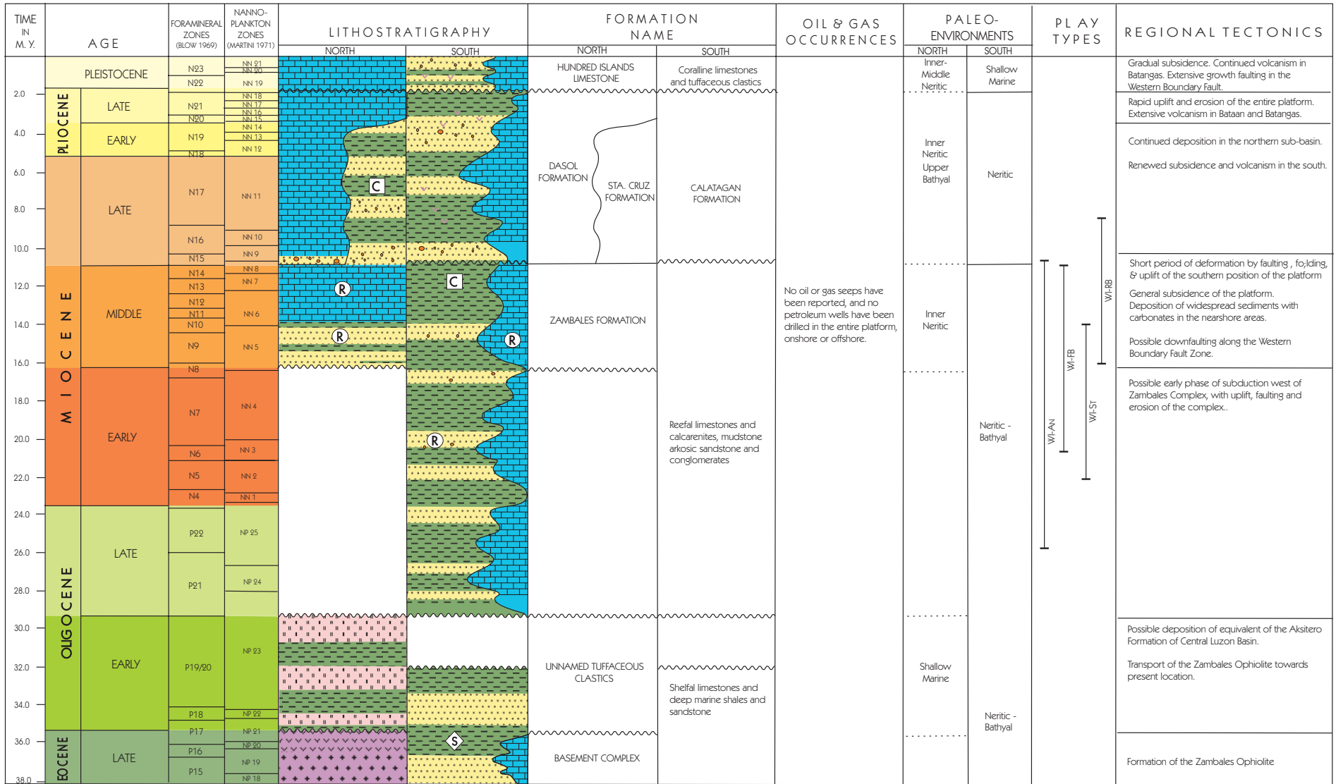
Stratigraphic Column of the West Luzon Basin
