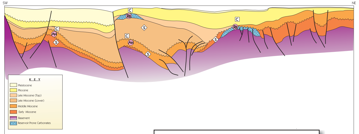
Schematic Play Concept Diagram for the Petroleum System in the Cotabato Basin
