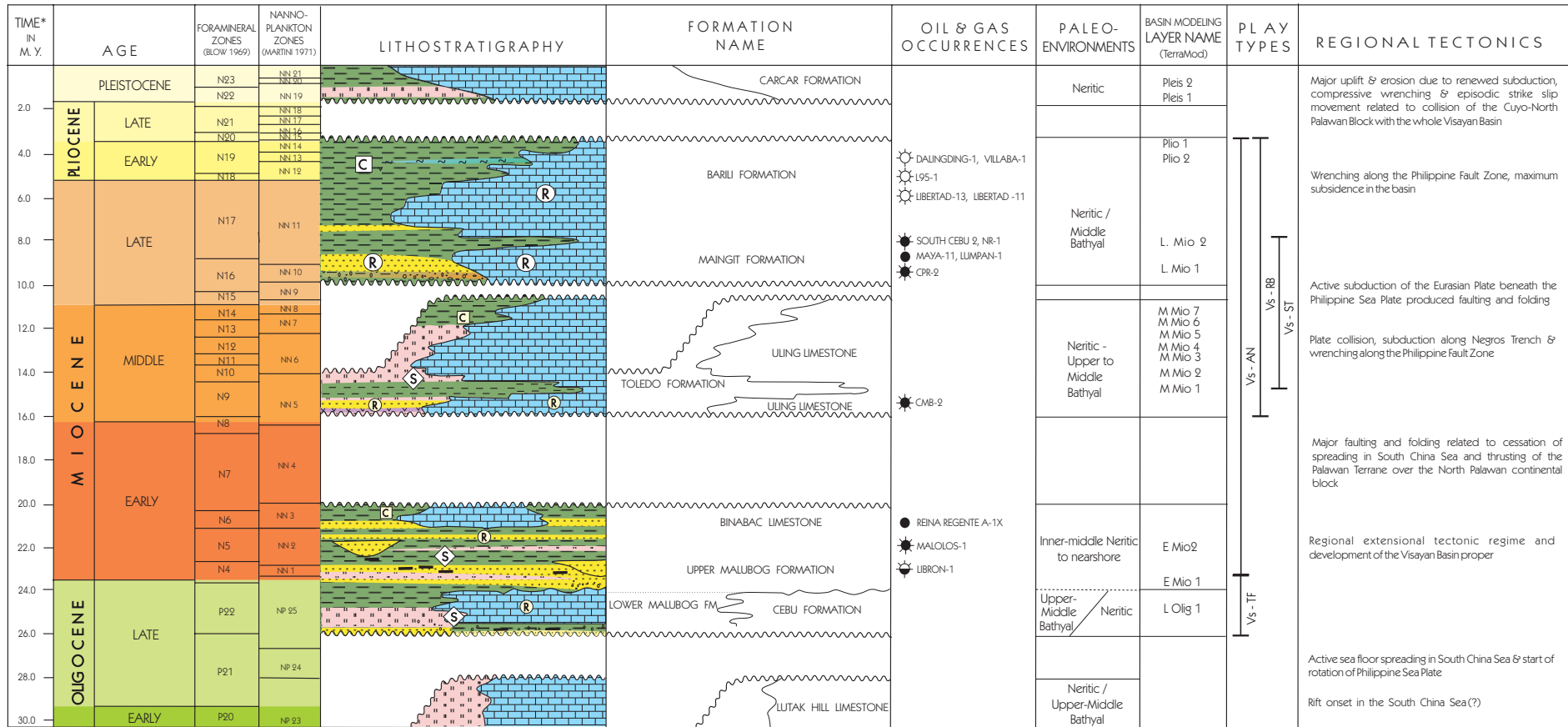
Stratigraphic Column of the Oligocene to Pleistocene Sedimentary Formations of the Visayan Basin
